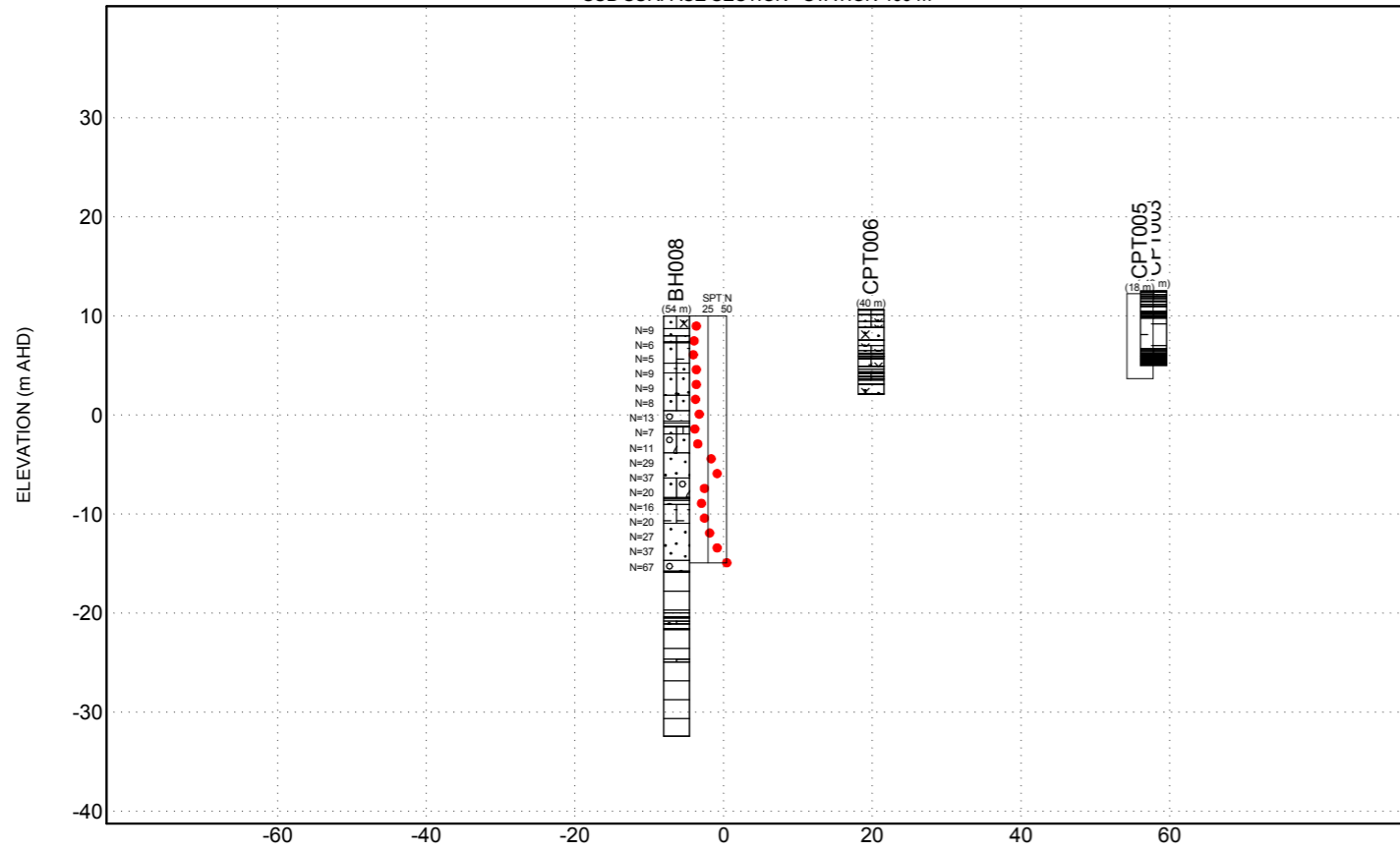
SUB SURFACE SECTION - STATION 400 m
